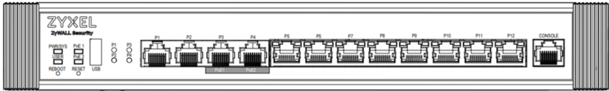
Figure 37 USG FLEX 700H Front Panel
