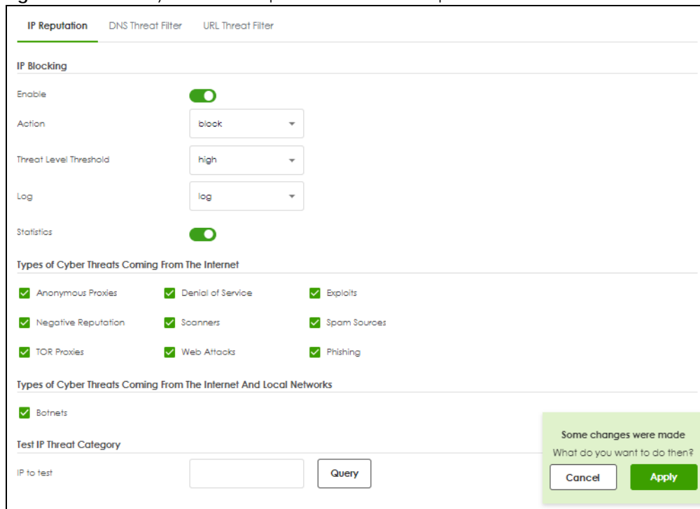
Figure 196 Security Service > Reputation Filter > IP Reputation
